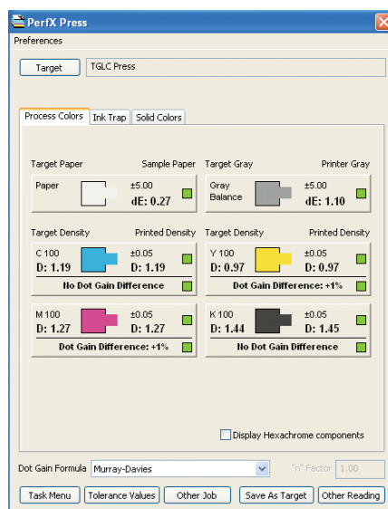
Status window.
